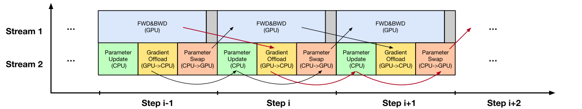
Fig. 10. An illustration of ZeRO-Offload and ZeRO-Offload with delayed parameter update.
